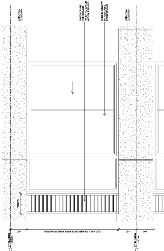
1 TYPICAL VERTICAL PLENUM - LEVEL 1 TO 4 1:20
