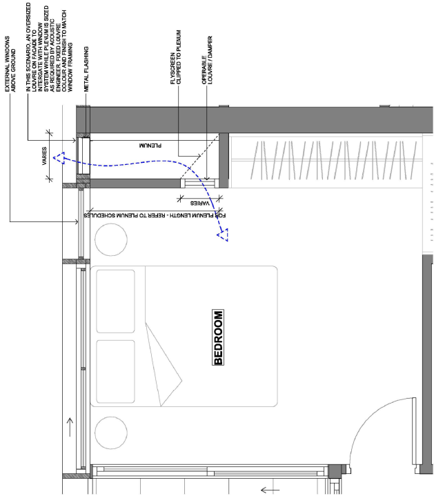
2 TYPICAL INTERNAL VERTICAL PLENUM - LEVEL 1 TO 4 1:20
